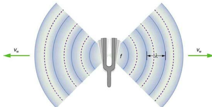
Figure 17.9 A sound wave emanates from a source vibrating at a frequency f , propagates at v_w , and has a wavelength \lambda .
