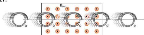
Figure 23.59 A coil is moved into and out of a region of uniform magnetic field. A coil is moved through a magnetic field as shown in Figure 23.59 . The field is uniform inside the rectangle and zero outside. What is the direction of the induced current and what is the direction of the magnetic force on the coil at each position shown?
