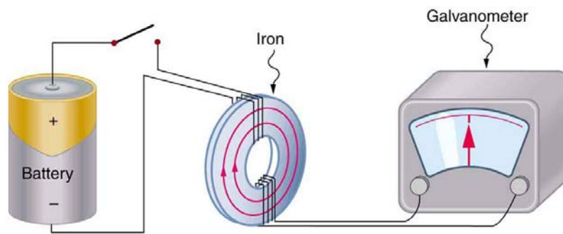
Figure 23.3 Faraday's apparatus for demonstrating that a magnetic field can produce a current. A change in the field produced by the top coil induces an emf and, hence, a current in the bottom coil. When the switch is opened and closed, the galvanometer registers currents in opposite directions. No current flows through the galvanometer when the switch remains closed or open.
