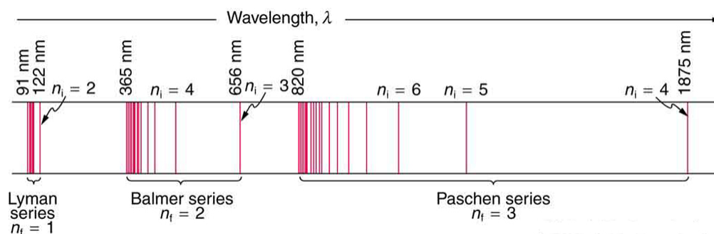
Figure 30.16 A schematic of the hydrogen spectrum shows several series named after those who contributed most to their determination. Part of the Balmer series is in the visible spectrum, while the Lyman series is entirely in the UV, and the Paschen series and others are in the IR. Values of n_f and n_i are shown for some of the lines.
