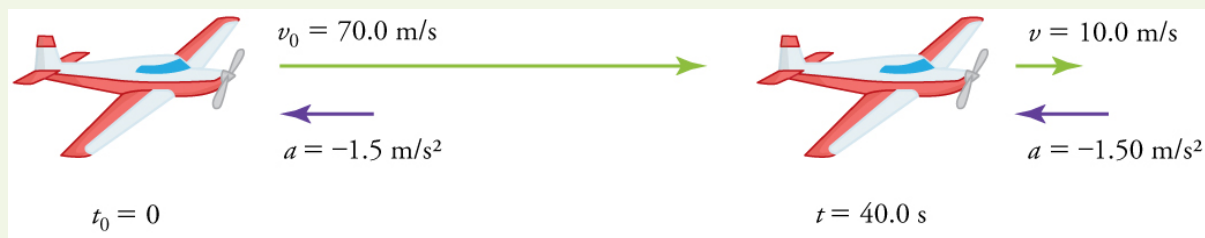
Figure 2.29 The airplane lands with an initial velocity of 70.0 m/s and slows to a final velocity of 10.0 m/s before heading for the terminal. Note that the acceleration is negative because its direction is opposite to its velocity, which is positive.
