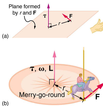
Figure 10.29 In figure (a), the torque is perpendicular to the plane formed by \mathbf{r} and \mathbf{F} and is the direction your right thumb would point to if you curled your fingers in the direction of \mathbf{F} . Figure (b) shows that the direction of the torque is the same as that of the angular momentum it produces.
