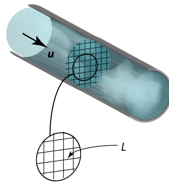
Figure 3.5: A simple mechanism for generating turbulence. A flow of water in a pipe (upstream velocity U ) flows through a mesh (spacing L ). If Re = UL/\nu is sufficiently large, the downstream flow becomes turbulent.
