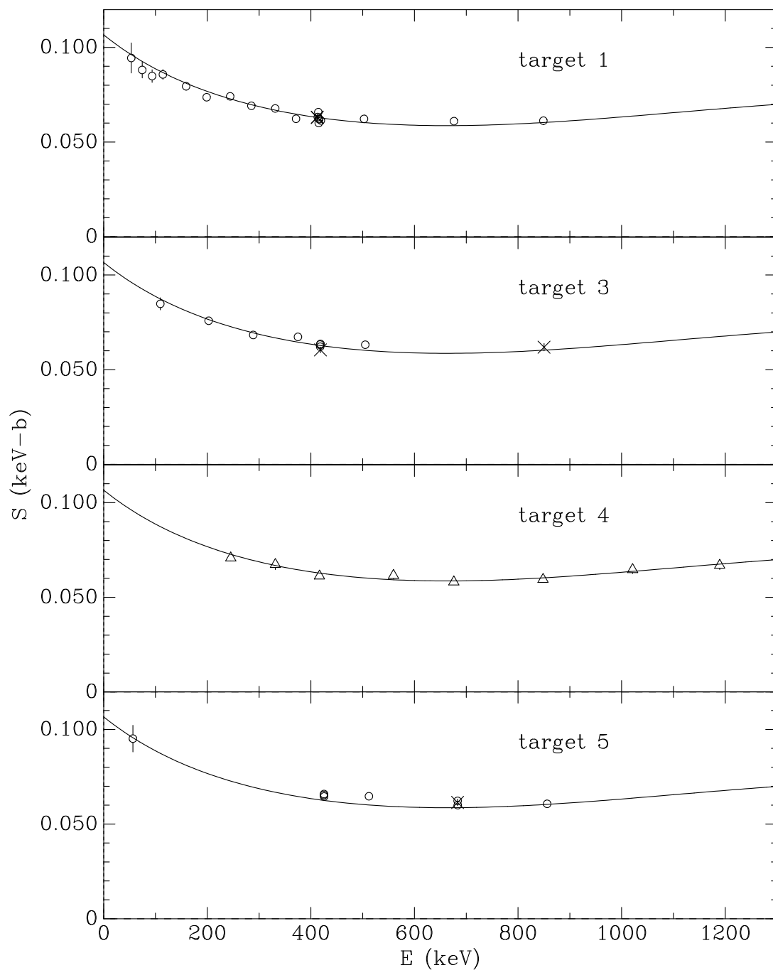
Figure 5.1: Total S-factors obtained from targets 1, 3-5. The circles, crosses and triangles correspond to data taken in geometries A, B, and C, respectively. The solid curves are Equation 1.16, normalized to S(0) = 0.1067 keV-b.
