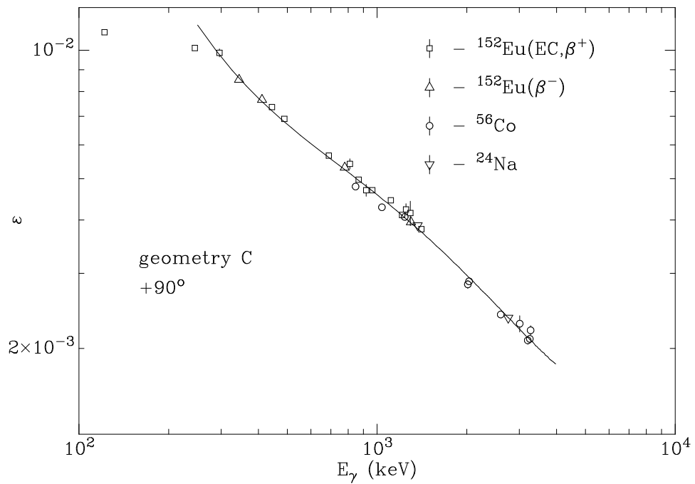
Figure E.6: Photopeak efficiency, geometry C, +90^\circ .
