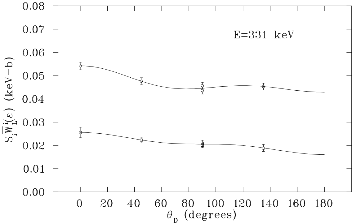
Figure F.3: E = 331 keV Angular Distribution.
