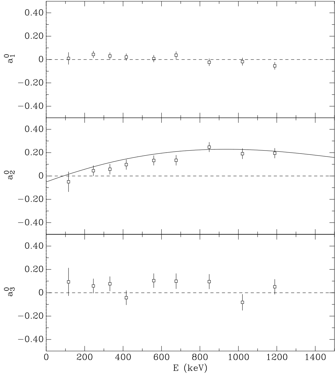
Figure 5.6: \gamma_0 angular-distribution coefficients. The errors are statistical; the systematic uncertainty in a_\ell^0 is estimated to be \pm 0.03 . The solid curve is the calculation of Tombrello and Parker [Tom63] for a_2^0 .
