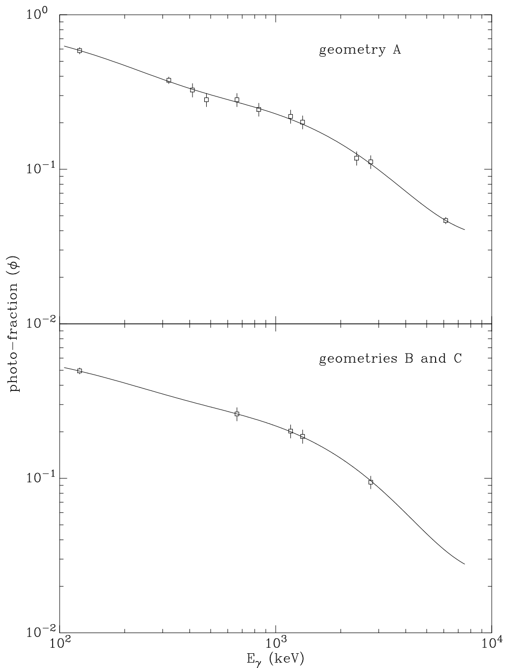
Figure 3.4: The photofraction for geometry A is shown in the upper panel. The squares are the experimental points, and solid line is the curve used in subsequent analysis. The squares on the lower panel are the experimental results for geometry B; the solid curve on the lower panel is used in the subsequent analysis for geometries B and C.
