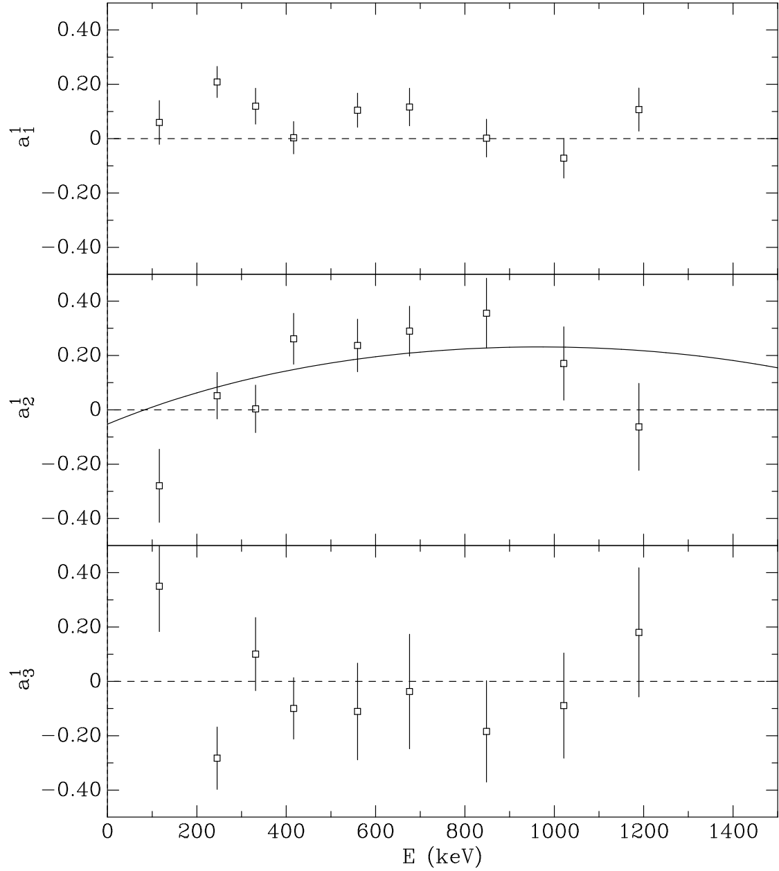
Figure 5.7: \gamma_1 angular-distribution coefficients. The errors are statistical; the systematic uncertainty in a_\ell^1 is estimated to be \pm 0.03 . The solid curve is the calculation of Tombrello and Parker [Tom63] for a_2^1 .
