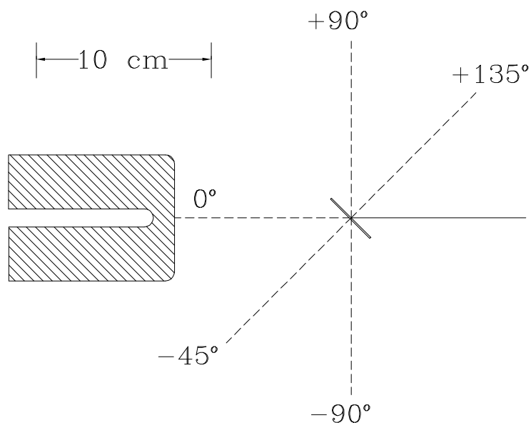
Figure 3.3: A scale diagram of geometry C, showing only the target and sensitive Ge.
