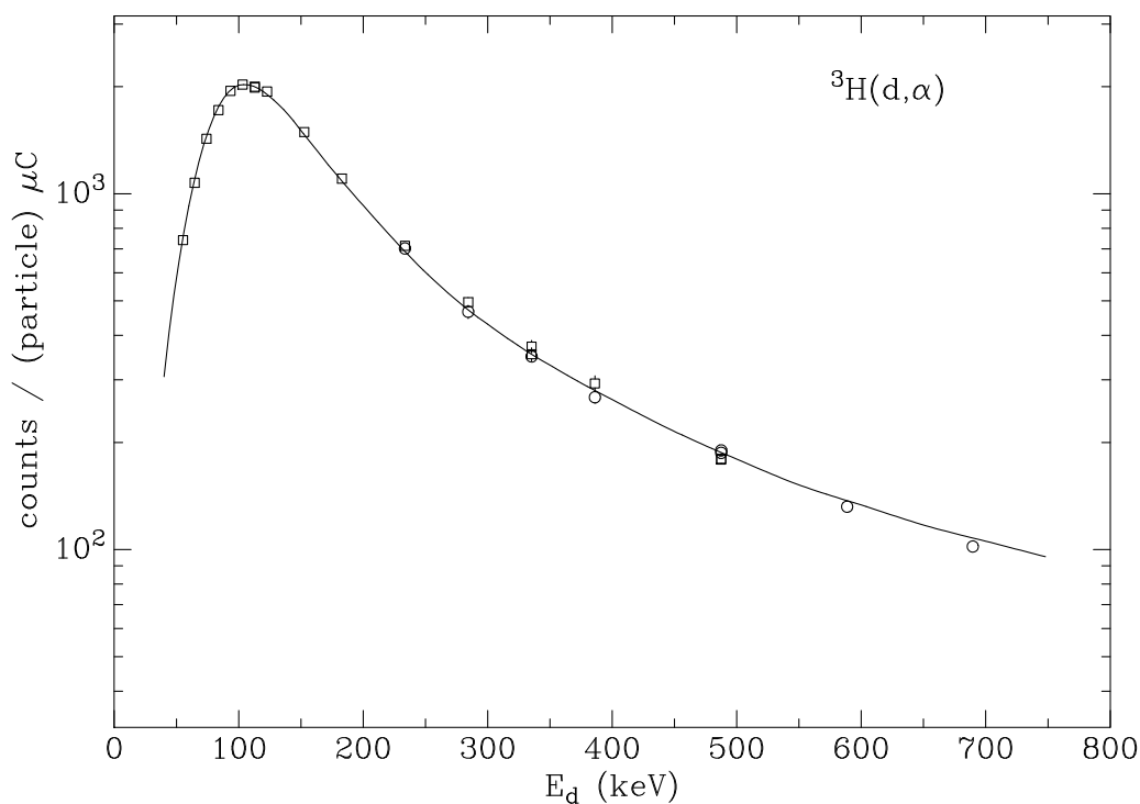
Figure 2.9: {}^3\text{H}(d, \alpha) excitation function obtained using deuteron (circles) and \text{D}_3^+ (squares) beams. The solid curve is the recommended cross section [Dro87], normalized to the data.
