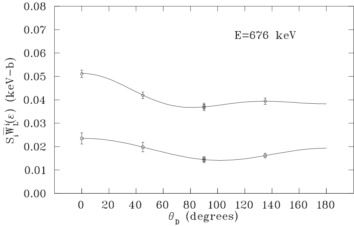
Figure F.6: E = 676 keV Angular Distribution.
