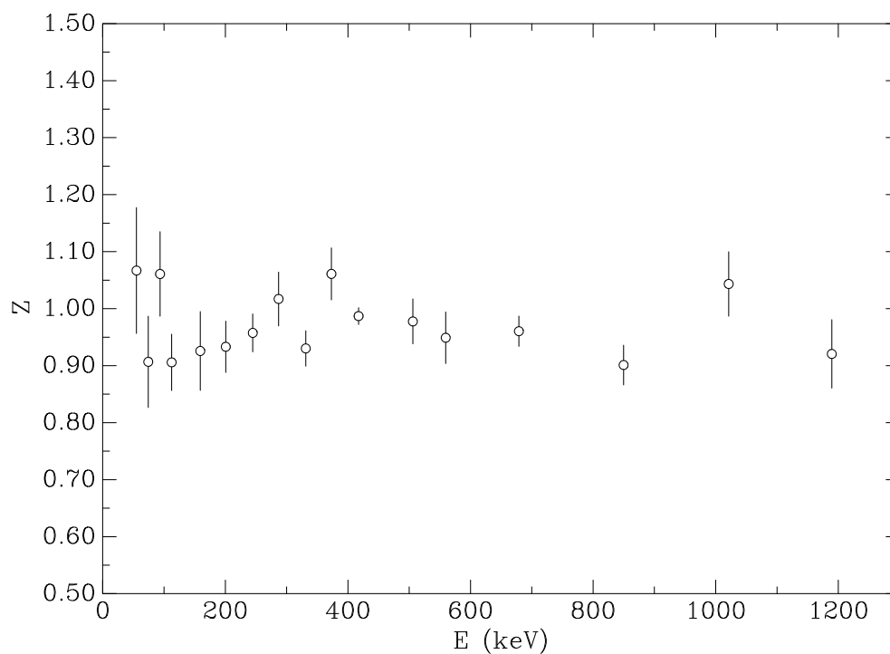
Figure 5.4: The ratio Z = \sigma_1/\sigma_2 ; the error bars include only statistical uncertainties. Note the suppressed zero.
