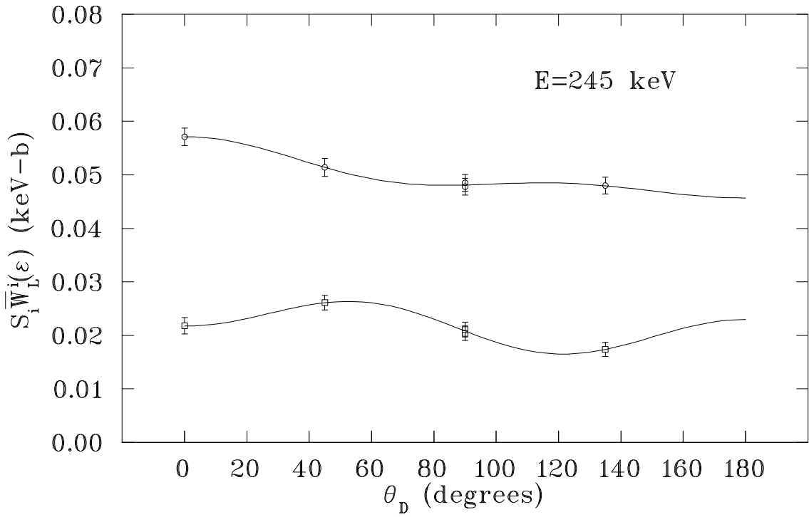
Figure F.2: E = 245 keV Angular Distribution.
