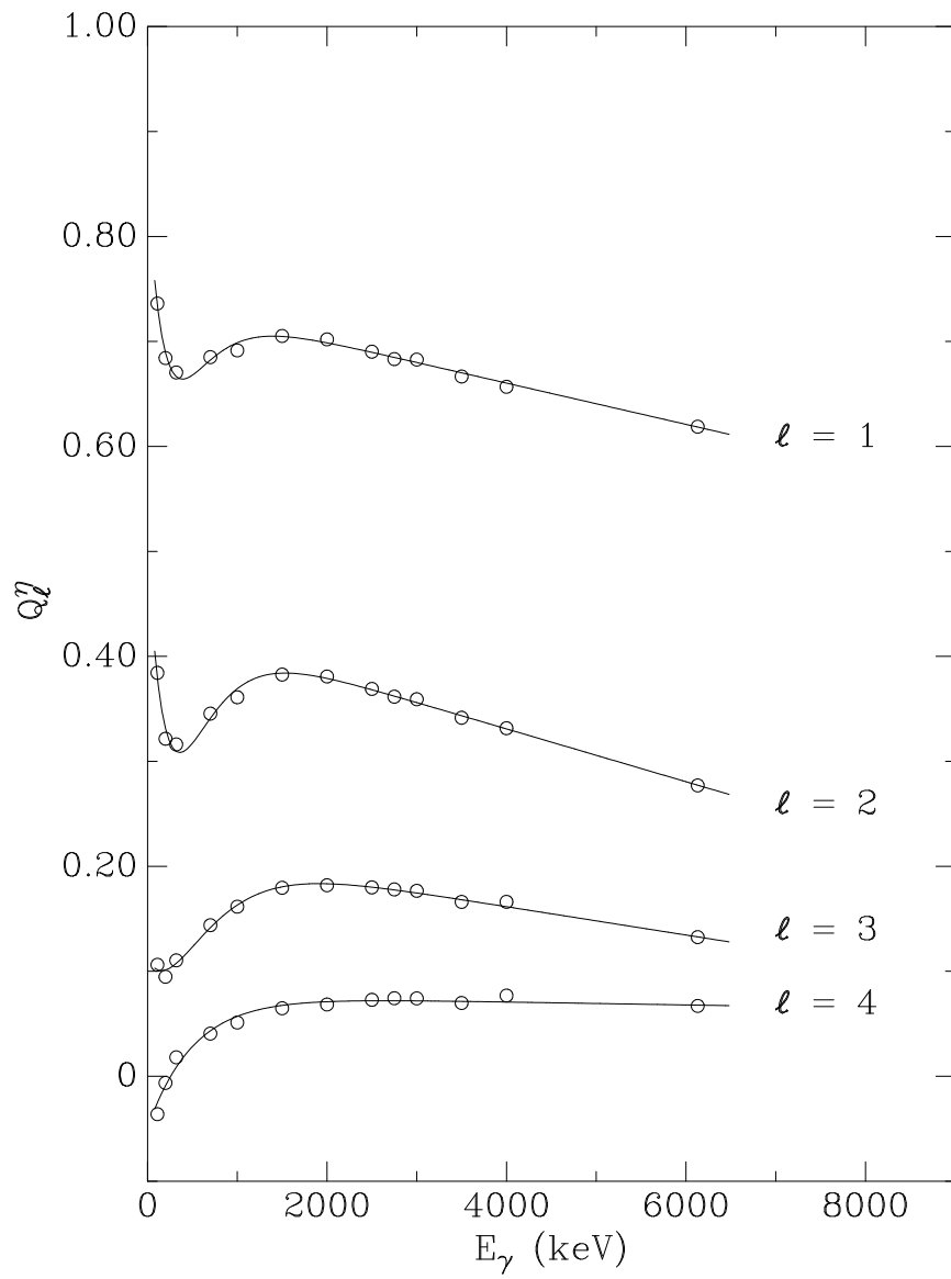
Figure D.4: Total attenuation factors, geometry A.
