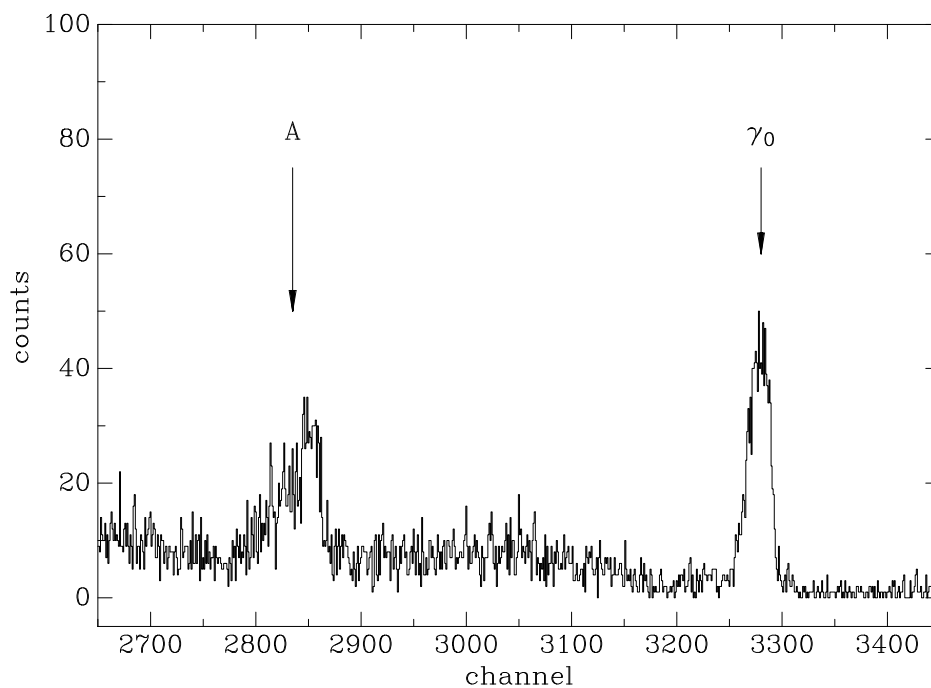
Figure 4.5: High-energy portion of run 137 spectrum obtained with target 4 and E_\alpha = 2790 keV, with the detector in the -90^\circ position. The \gamma_0 transition is cleanly resolved, but the \gamma_1 transition and the first-escape peak from the \gamma_0 transition overlap (peak A). The energy calibration is different from runs 095 and 096 (Figures 4.1–4.4).
