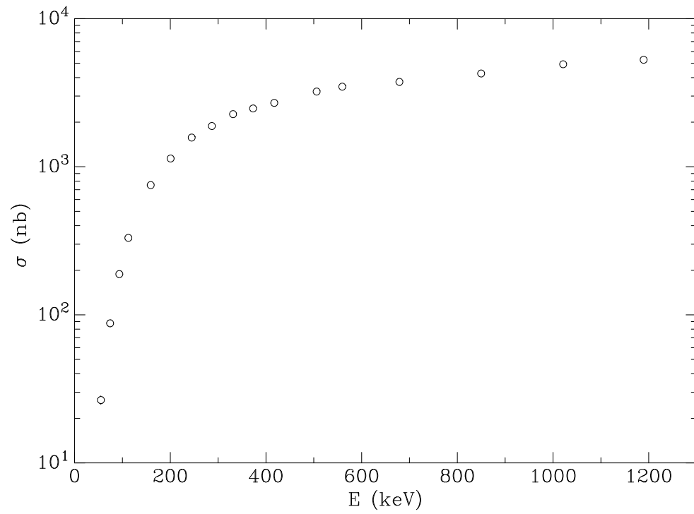
Figure 5.2: The final result for \sigma , found by combining data sets shown in Figure 5.1.
