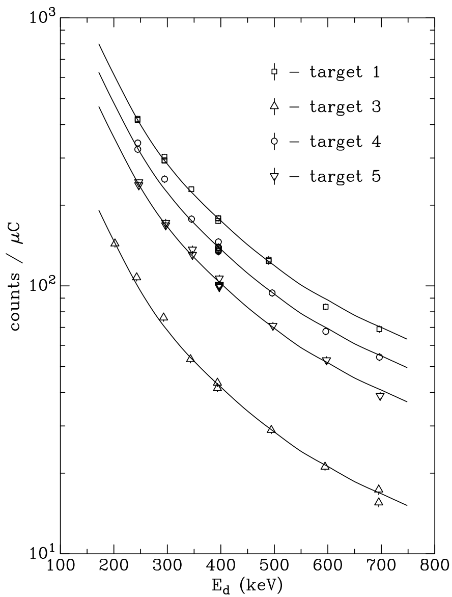
Figure 2.8: {}^3\text{H}(d, \alpha) excitation functions obtained from targets 1, 3–5. The solid curves are the recommended cross sections [Dro87], normalized to the data.
