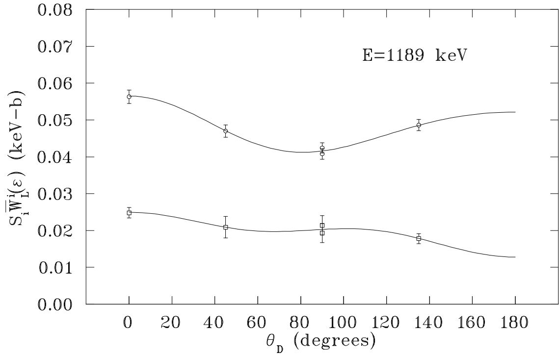
Figure F.9: E = 1189 keV Angular Distribution.
