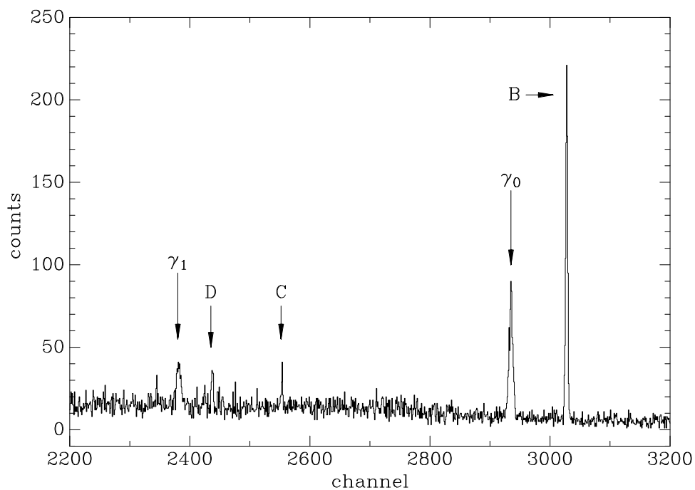
Figure 4.1: High-energy portion of run 096 spectrum obtained with target 5 and E_\alpha = 140 keV, showing the \gamma_0 and \gamma_1 transitions. The peak labeled B is a background line at 2614 keV from ^{208}\text{Tl} decay ( ^{232}\text{Th} decay product). Peak C is a background line at 2204 keV from ^{214}\text{Bi} decay ( ^{226}\text{Ra} decay product). Peak D is the first-escape peak associated with peak B.
