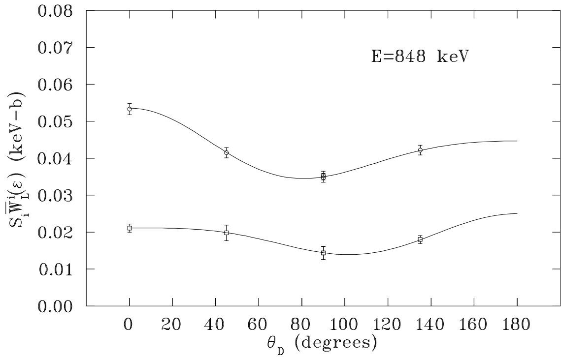
Figure F.7: E = 848 keV Angular Distribution.
