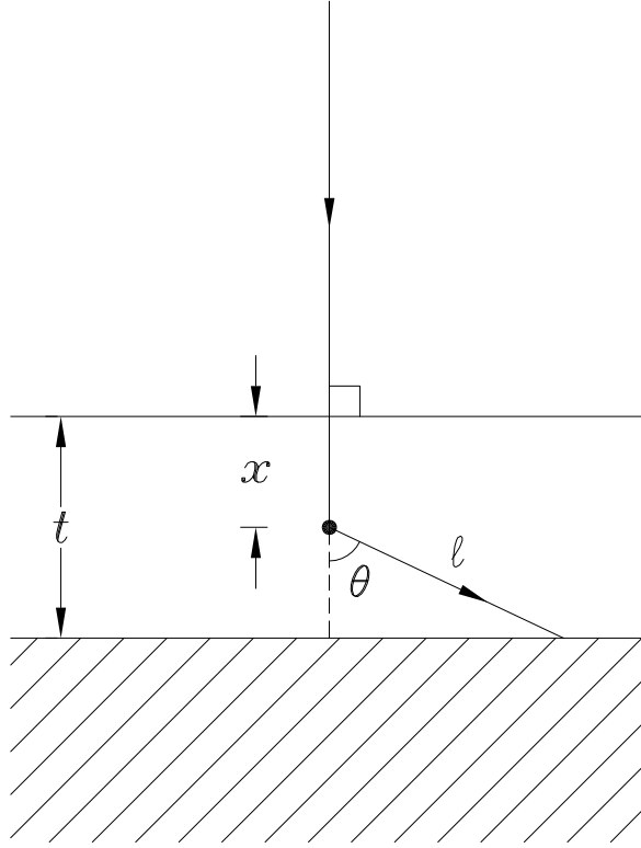
Figure B.1: Definition of variables for the normally incident case. The target is viewed perpendicular to normal.
