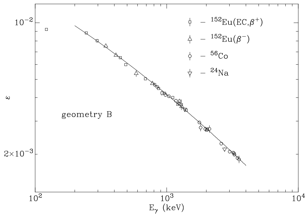
Figure E.2: Photopeak efficiency, geometry B.
