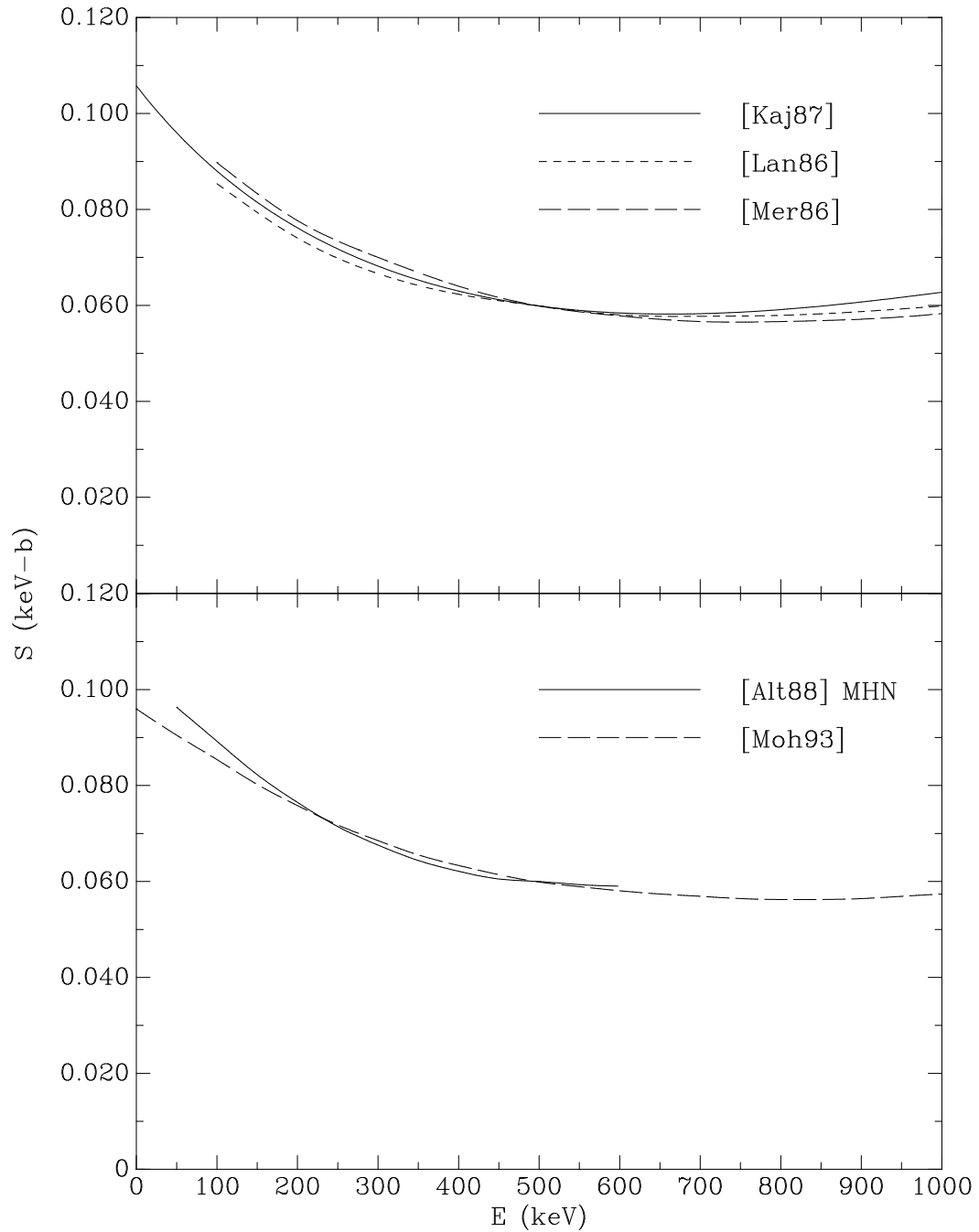
Figure 1.7: Theoretical calculations of S(E) for {}^3\text{H}(\alpha, \gamma){}^7\text{Li} by Kajino, Toki, and Austin [Kaj87], Langanke [Lan86], Mertelmeier and Hofmann [Mer86], Altmeyer et al. [Alt88], and Mohr et al. [Moh93]. We have used the Modified Hasegawa-Nagata (MHN) interaction calculation of Altmeyer et al. The curves have been normalized to S(500 \text{ keV}) = 0.060 \text{ keV-b} .
