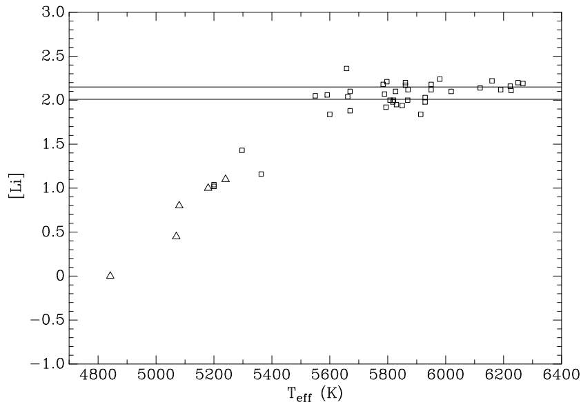
Figure 1.2: Observed Li abundance versus T_{eff} , for the most metal-poor stars ( [\text{Fe}/\text{H}] \leq -1.3 ). The diamonds are upper limits to [\text{Li}] . The horizontal lines correspond to Equation 1.7. (Adapted from Walker et al. [Wal91].)
