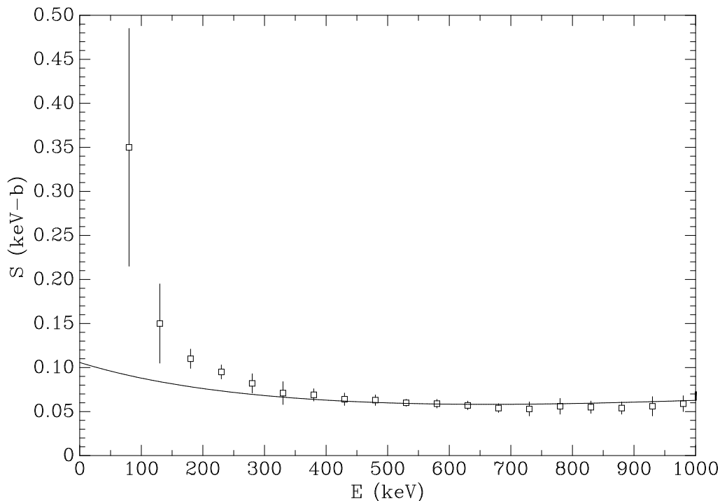
Figure 1.6: The Coulomb dissociation results of Utsunomiya et al. [Uts90]. The solid curve is Equation 1.16, normalized to S(500 \text{ keV}) = 0.060 \text{ keV-b} . Note that the vertical scale has been expanded compared to Figure 1.5.
