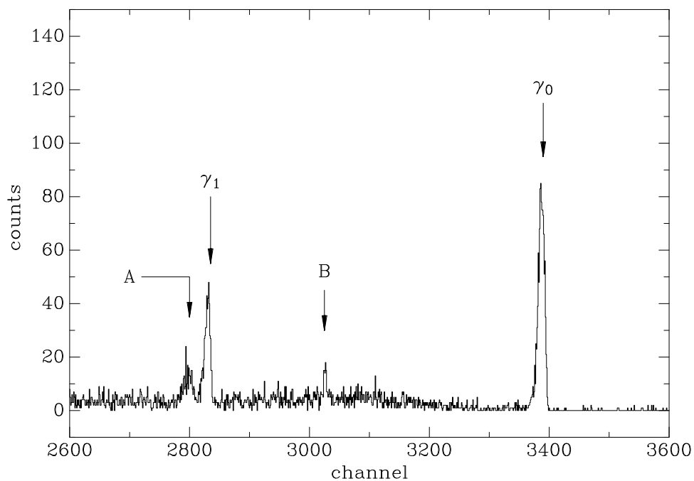
Figure 4.3: High-energy portion of run 095 spectrum obtained with target 5 and E_\alpha = 1000 keV, showing the \gamma_0 and \gamma_1 transitions. The peak labeled A is the \gamma_0 first-escape peak; peak B is a background line at 2614 keV from ^{208}\text{Tl} decay ( ^{232}\text{Th} decay product). The energy calibration is the same as for run 096 (Figures 4.1 and 4.2).
