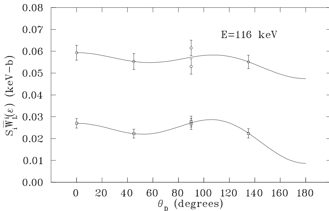
Figure F.1: E = 116 keV Angular Distribution.
