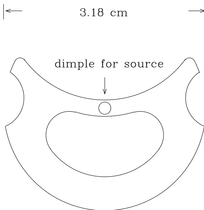
Figure 2.3: Top view of the Ta boats. The Ti evaporation source is placed in the hemispherical dimple at the center.
