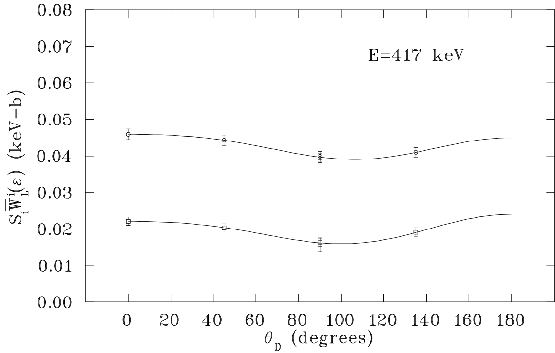
Figure F.4: E = 417 keV Angular Distribution.
