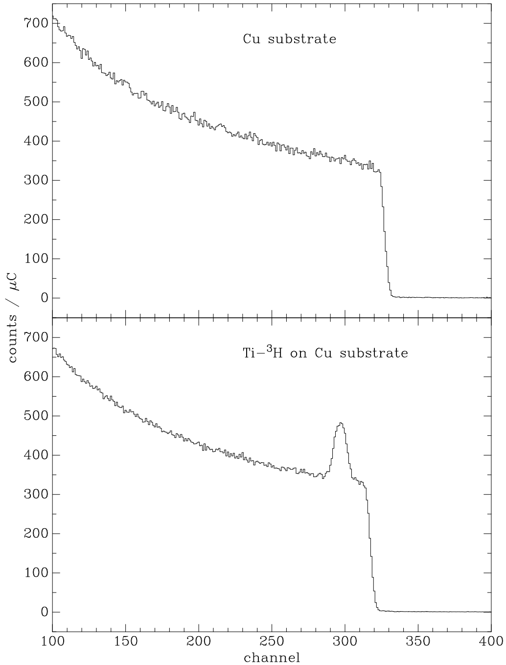
Figure 2.5: Spectra of scattered 2000-keV \alpha particles observed at \theta_{\text{lab}} = 165^\circ , from a blank Cu substrate (top panel) and target 1, a \text{Ti-}^3\text{H} layer on Cu substrate (bottom panel). The peak in the bottom panel at channel \approx 295 is from the Ti layer. The leading edge of the Cu-scattering plateau in the lower panel is shifted by 10.0 channels due to the presence of the \text{Ti-}^3\text{H} layer.
