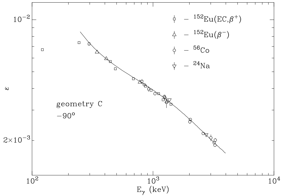
Figure E.5: Photopeak efficiency, geometry C, -90^\circ .
