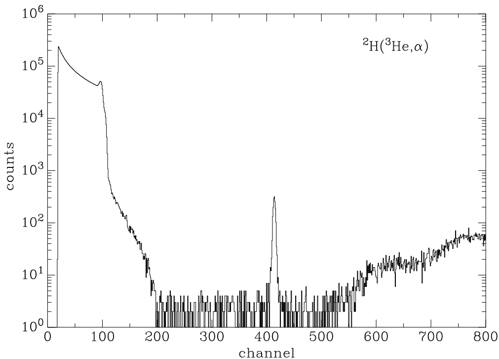
Figure 2.6: Si-detector spectrum resulting from the 650-keV- ^3\text{He} bombardment of Ti- ^2\text{H} on Cu substrate. The peak at channel \approx 415 is due to \alpha particles from the ^2\text{H}(^3\text{He}, \alpha) reaction. The counts in channels \geq 550 are due to high-energy protons from ^2\text{H}(^3\text{He}, p) that deposited a fraction of their energy in the detector.
