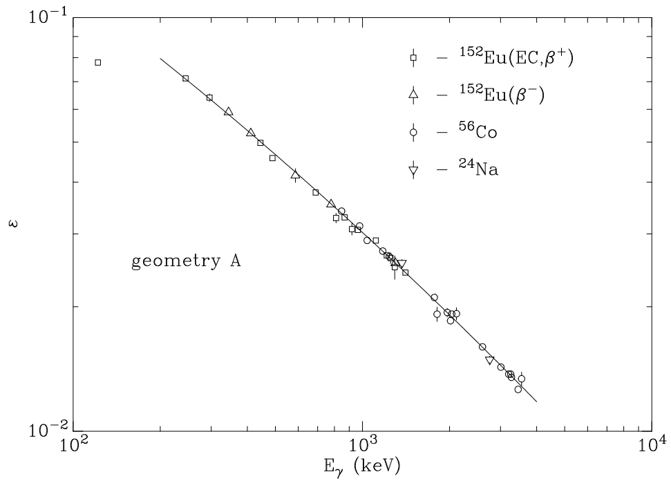
Figure E.1: Photopeak efficiency, geometry A.
