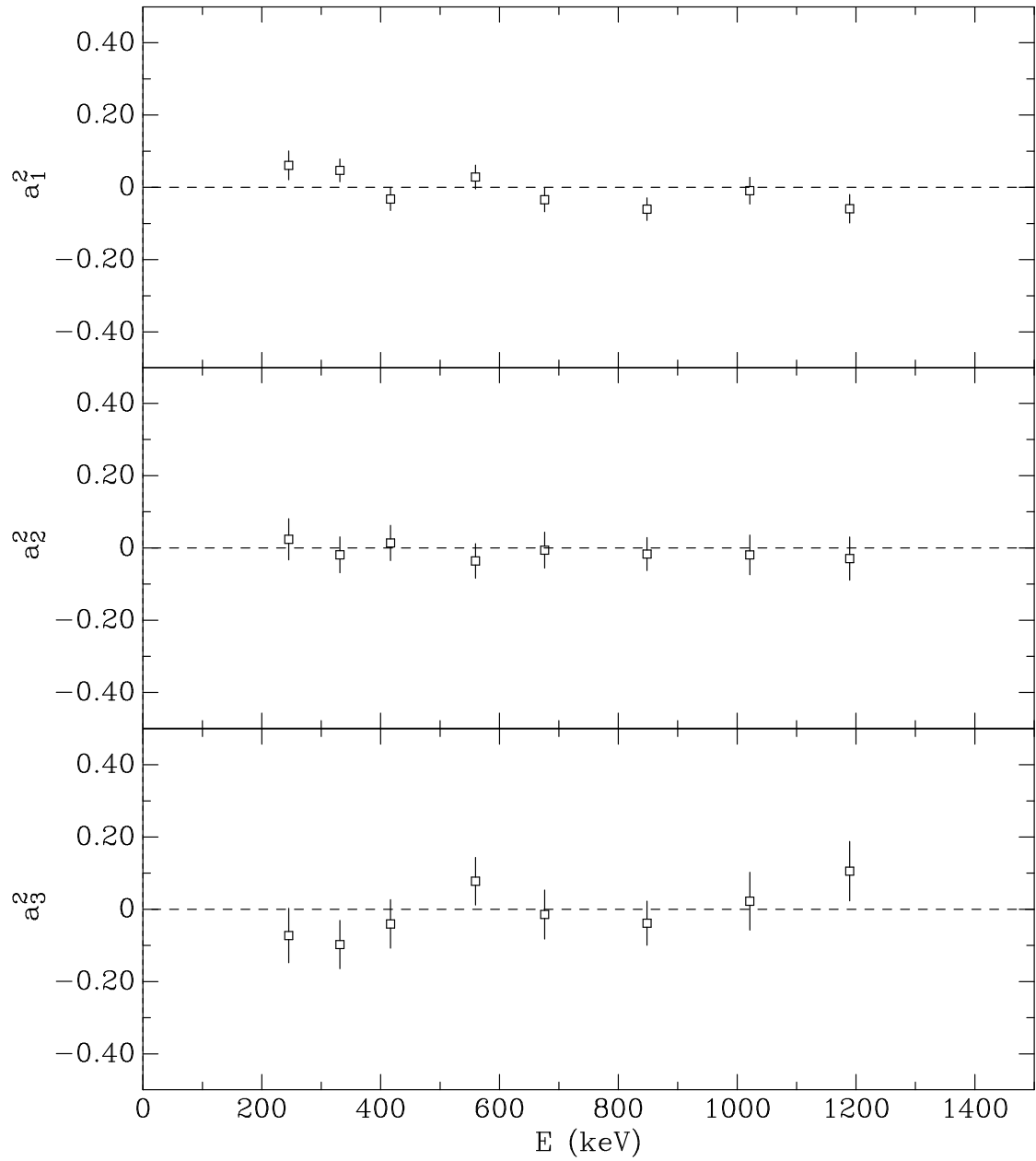
Figure 5.8: \gamma_2 angular-distribution coefficients. The errors are statistical; the systematic uncertainty in a_\ell^2 is estimated to be \pm 0.03 .
