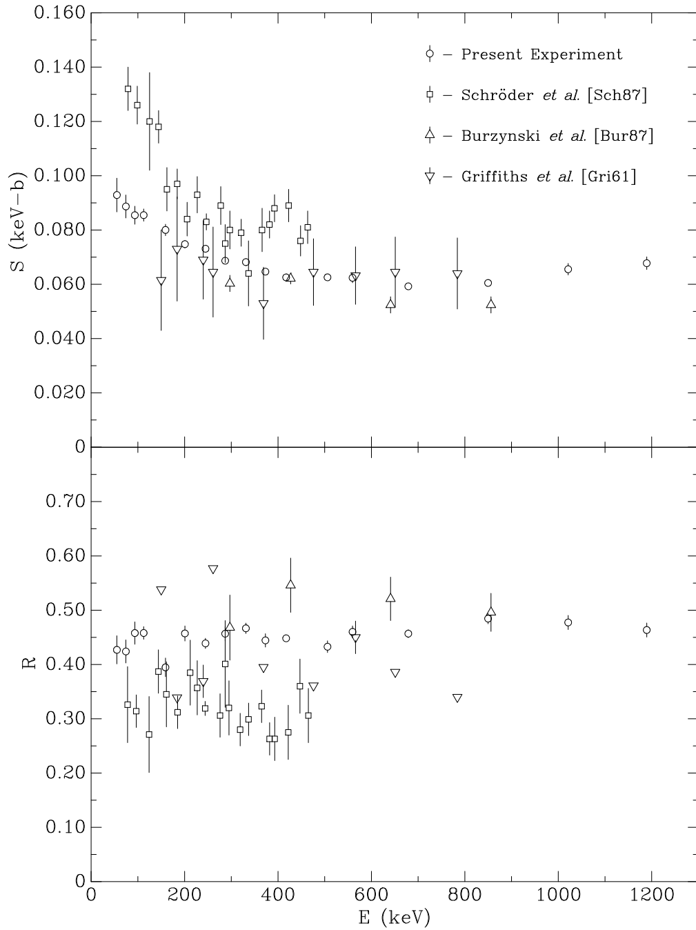
Figure 5.9: The present results for S and R , compared to previous direct measurements.
