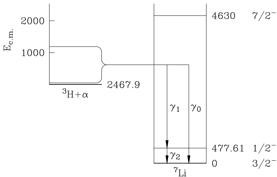
Figure 1.4: {}^7\text{Li} energy level diagram (all energies are given in keV).
