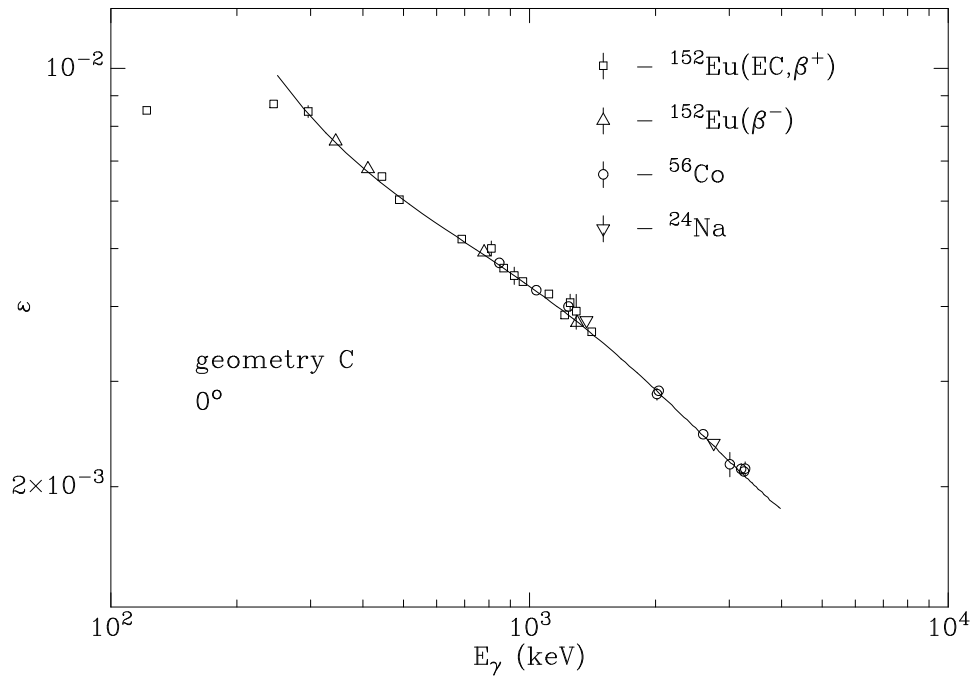
Figure E.3: Photopeak efficiency, geometry C, 0^\circ .
