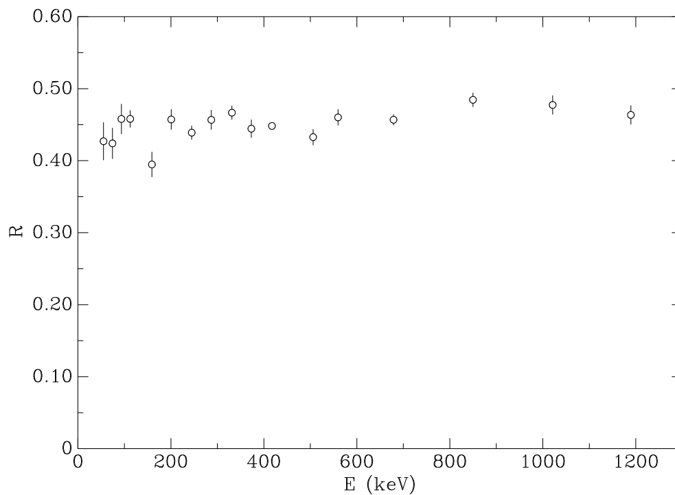
Figure 5.5: The branching ratio R . The error bars are statistical; the systematic error is estimated to be 4%.
