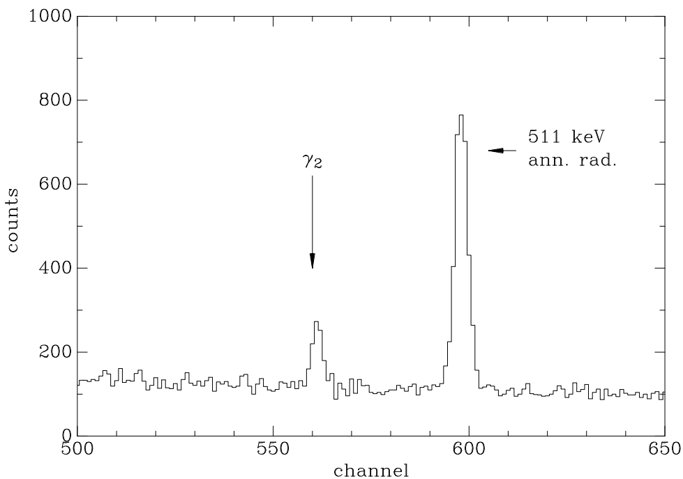
Figure 4.2: Low-energy portion of run 096 spectrum, showing the \gamma_2 transition and the 511-keV positron annihilation peak.
