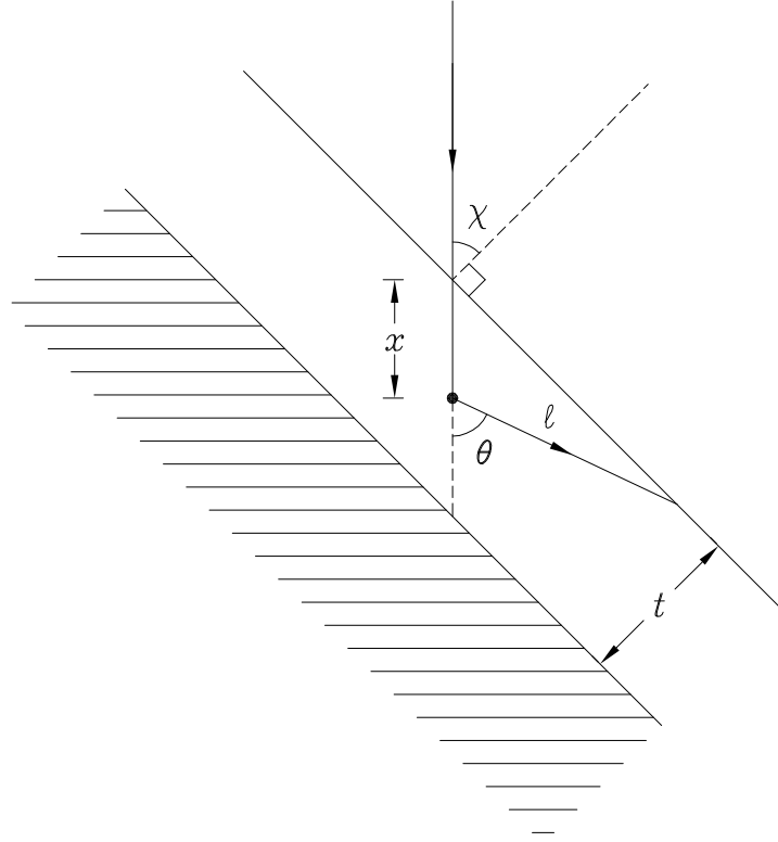
Figure B.3: Definition of variables for arbitrary angle of incidence. The target is viewed perpendicular to normal. Note that the distance \ell is not necessarily in the plane of the paper.
