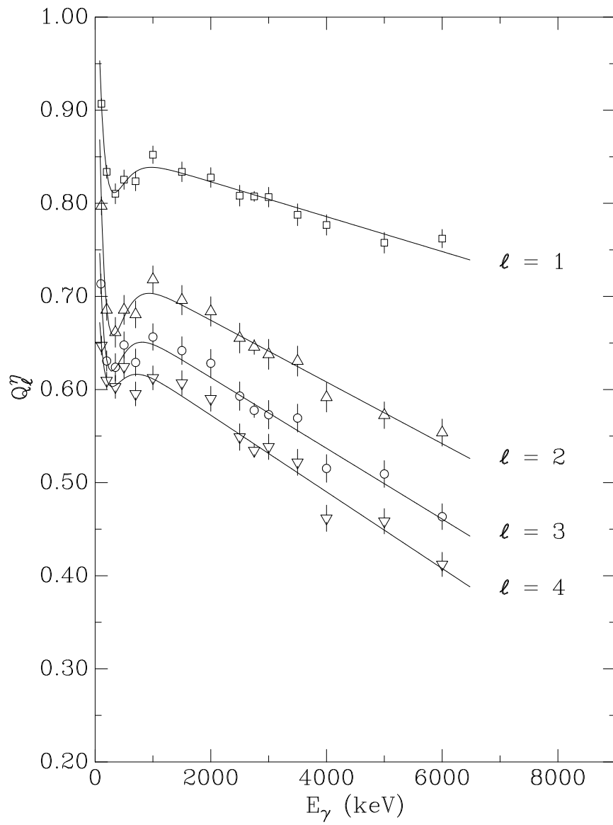
Figure D.5: Total attenuation factors, geometry B.
