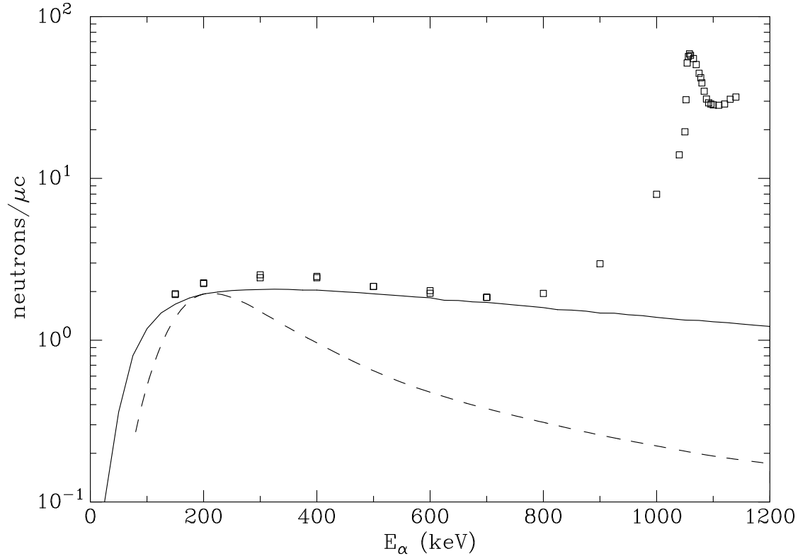
Figure B.4: The neutron yield is shown as a function of the incident E_\alpha , with the target at 45^\circ with respect to the incident beam. The squares are the experimental points. The solid curve is the calculation including energy loss (Equation B.15). The meaning of the dashed curve is described in the text.
