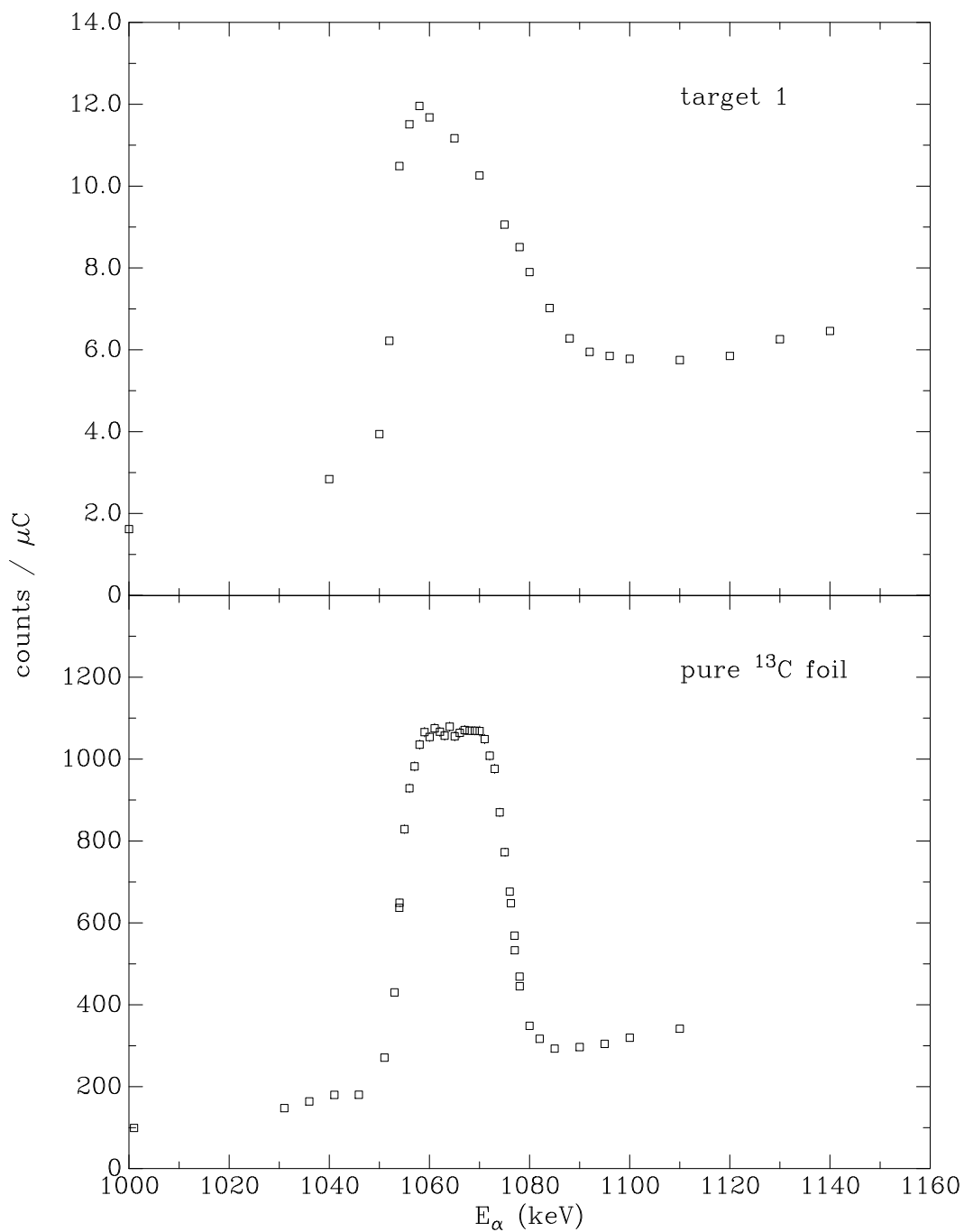
Figure 3.6: The ^{13}\text{C}(\alpha, n) yields are shown in the vicinity of the 1053-keV resonance. The upper panel is the result for target 1; the lower for a pure ^{13}\text{C} foil. Note that natural carbon is \approx 1.1\% ^{13}\text{C} .
