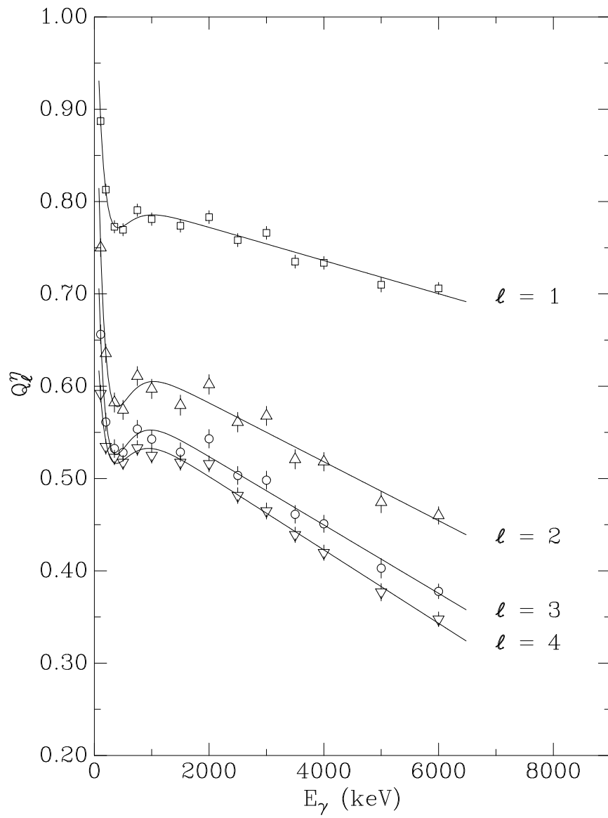
Figure D.6: Total attenuation factors, geometry C.
