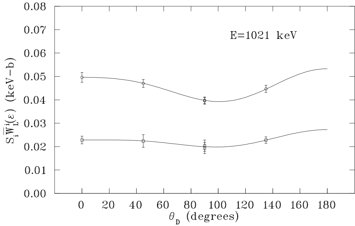
Figure F.8: E = 1021 keV Angular Distribution.
