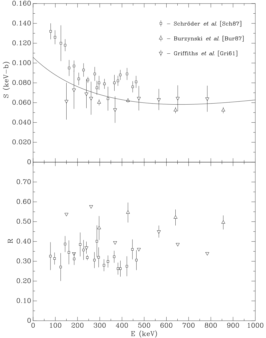
Figure 1.5: The previous results [Sch87, Bur87, Gri61] for S and R as a function of the center-of-mass energy E . The errors on the S data points of Schröder et al. and Burzynski et al. do not include respective systematic errors of 15% and 14%. Griffiths et al. only quoted uncertainties for a few R data points. The solid curve in the upper panel is Equation 1.16, normalized to S(500 \text{ keV}) = 0.060 \text{ keV-b} .
