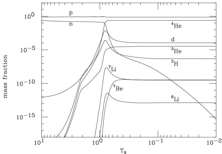
Figure 1.1: Evolution of the light-element abundances with temperature (measured in GK) in the big bang, for \eta_{10} = 3.0 .
