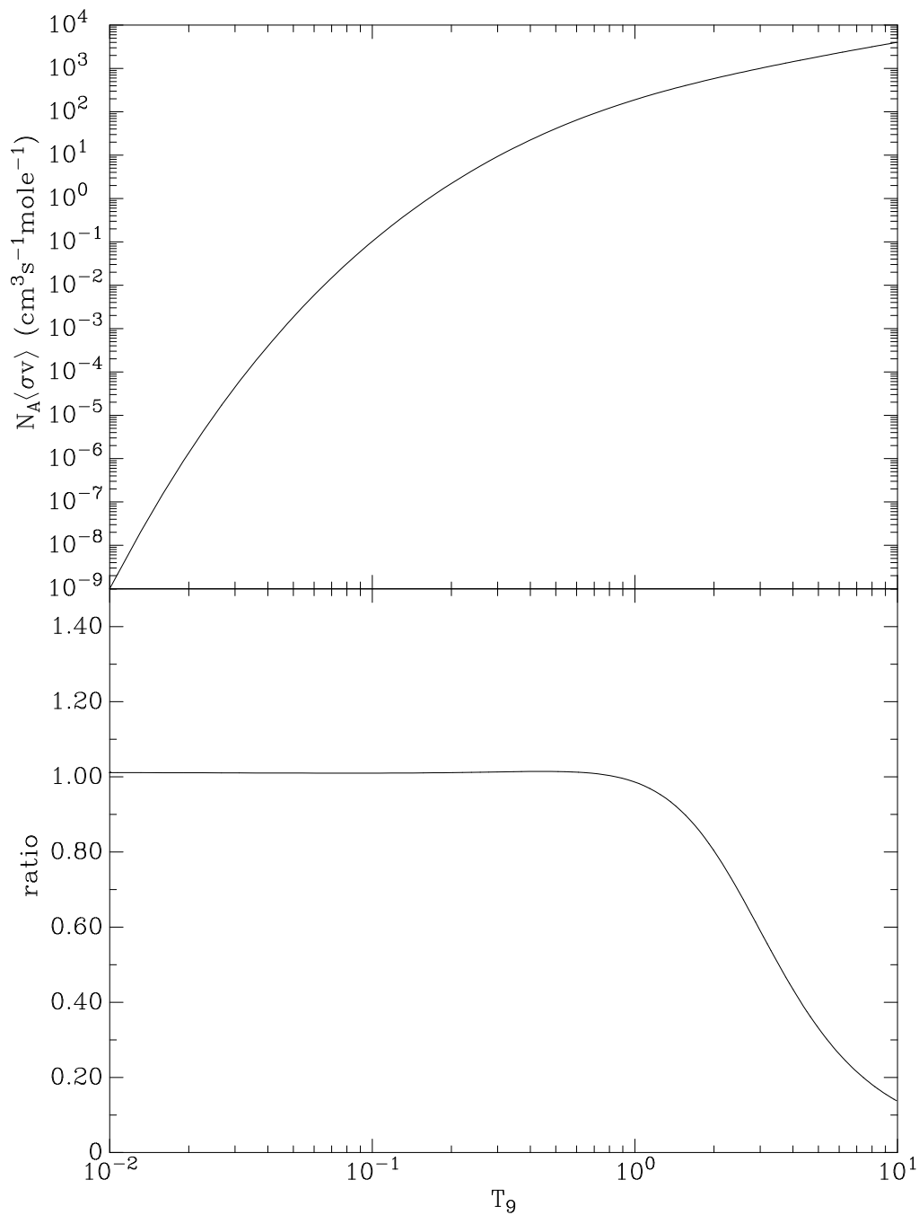
Figure 6.1: The thermonuclear reaction rate N_A \langle \sigma v \rangle calculated from our data is shown as a function of temperature in GK in the upper panel. The ratio of the present reaction rate to that given by Caughlan and Fowler [Cau88] is shown in the lower panel.
